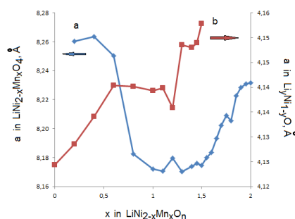
Fig. 1 Dependence of the lattice constant of spinel (a) and \text{Li}_y\text{Ni}_{1-y}\text{O} phase (b) on the total composition of \text{LiNi}_{2-x}\text{Mn}_x\text{O}_n system
